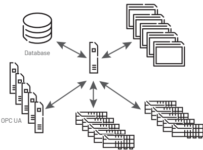
Figure 16. XL System architecture
